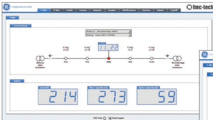
Application displays current line loading and available capacity based on the CIGRE algorithm
