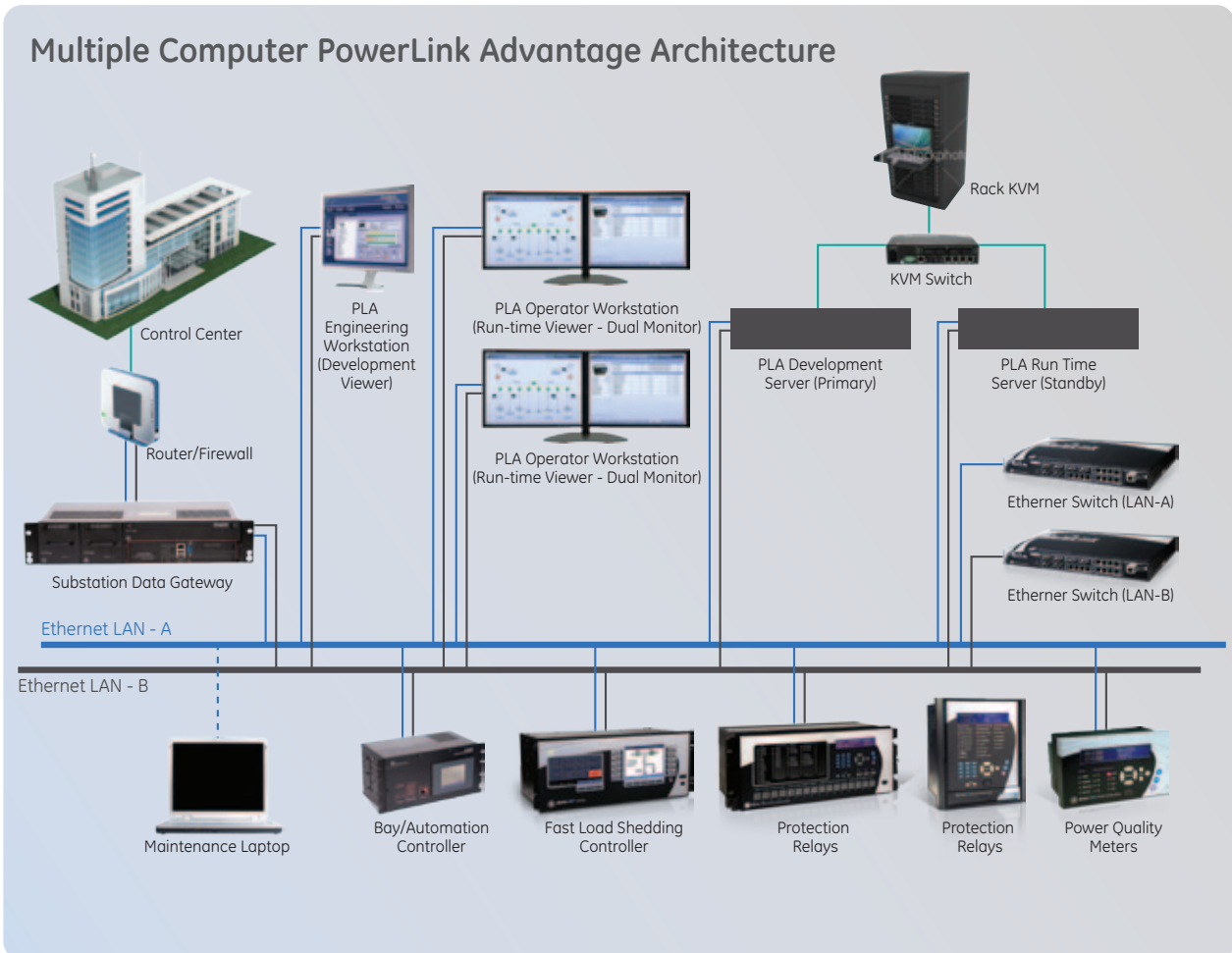
PLA server redundancy to ensure continuous uptime.
