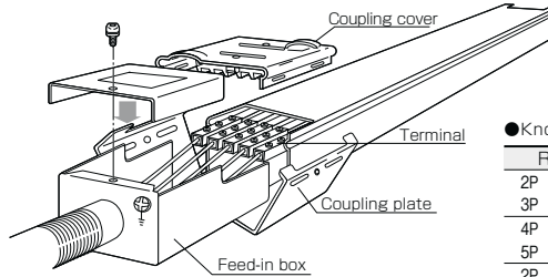
(Drawing shows a 5P Trolley Duct.)
