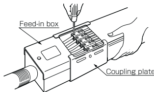
(Drawing shows a 5P Trolley Duct.)
