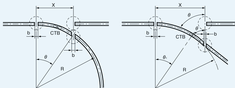
CTB: Center feed-in box
