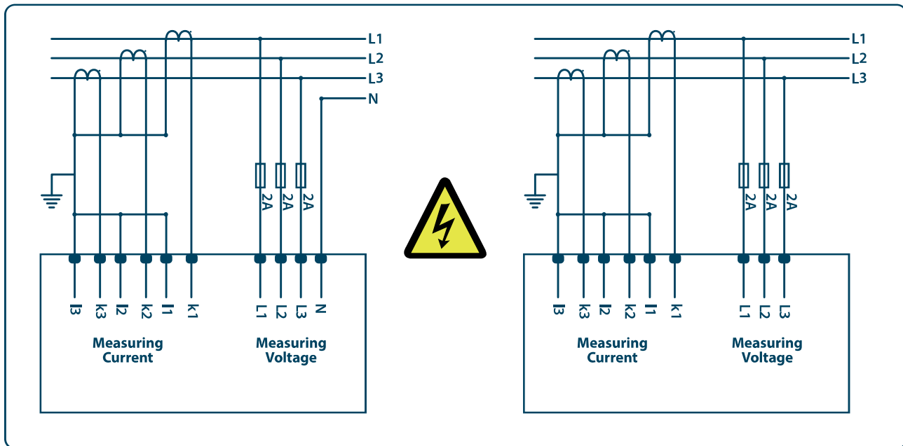
Figure 2-1 Connection Diagram
