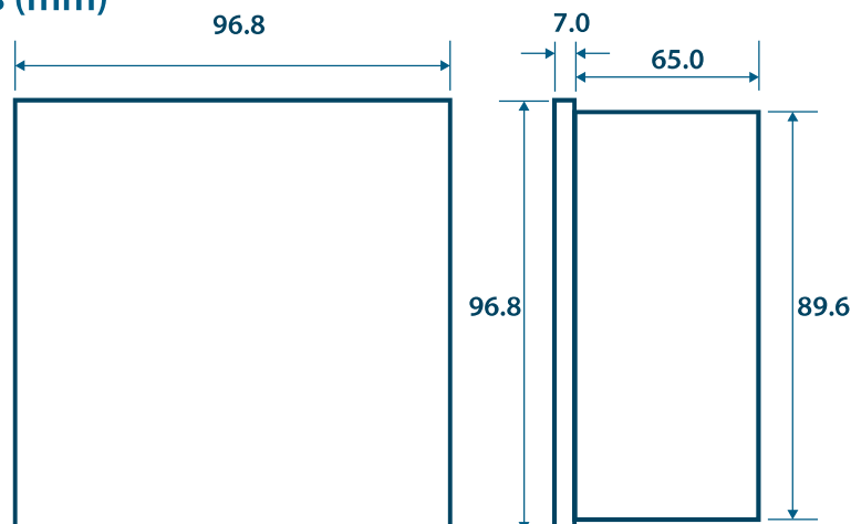
Figure 2-3 Dimensions for EMG 10
