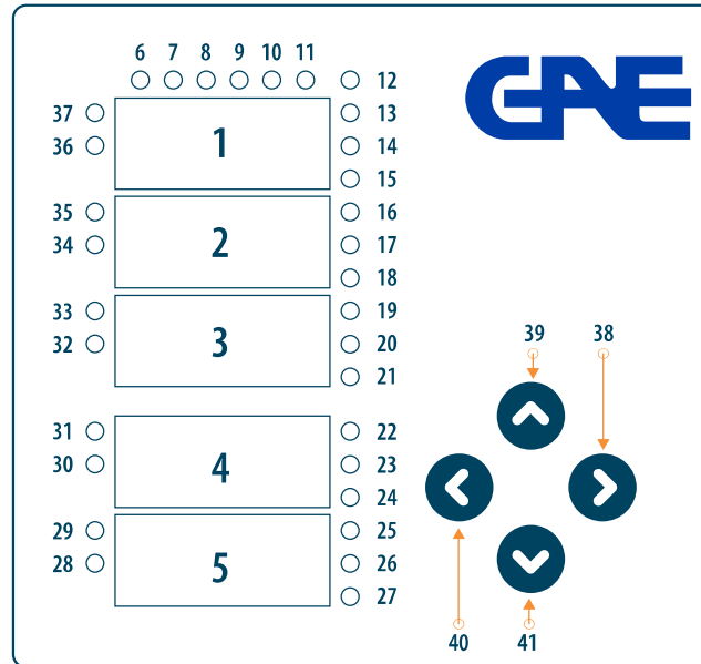
Figure 1-1 EMG 10 Front Panel
