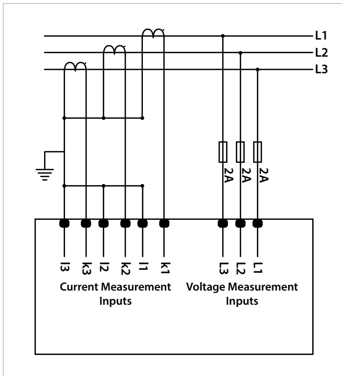
Figure 2-7 EMG 50 3 Phase Delta Connection Diagram
