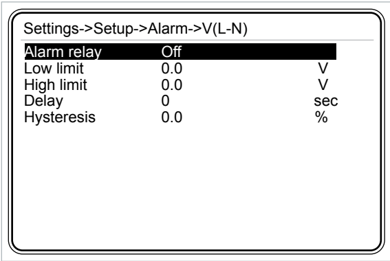
Figure 3-48 V(L-N) Menu
