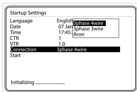
Figure 3-8 Connection Types
