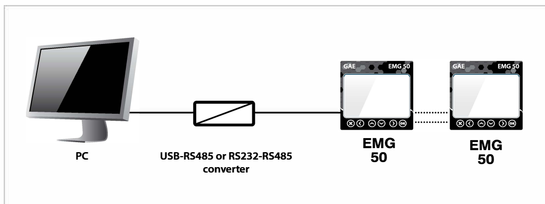
Figure 4-2 Connection of EMG 50 to a PC
