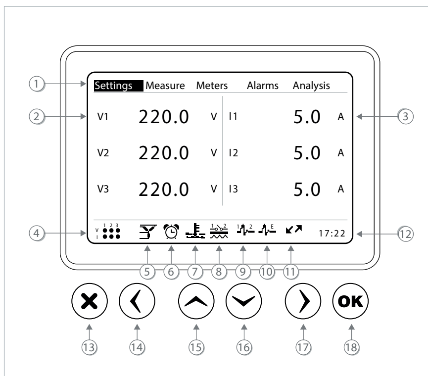
Figure 1-1 EMG 50 Display
