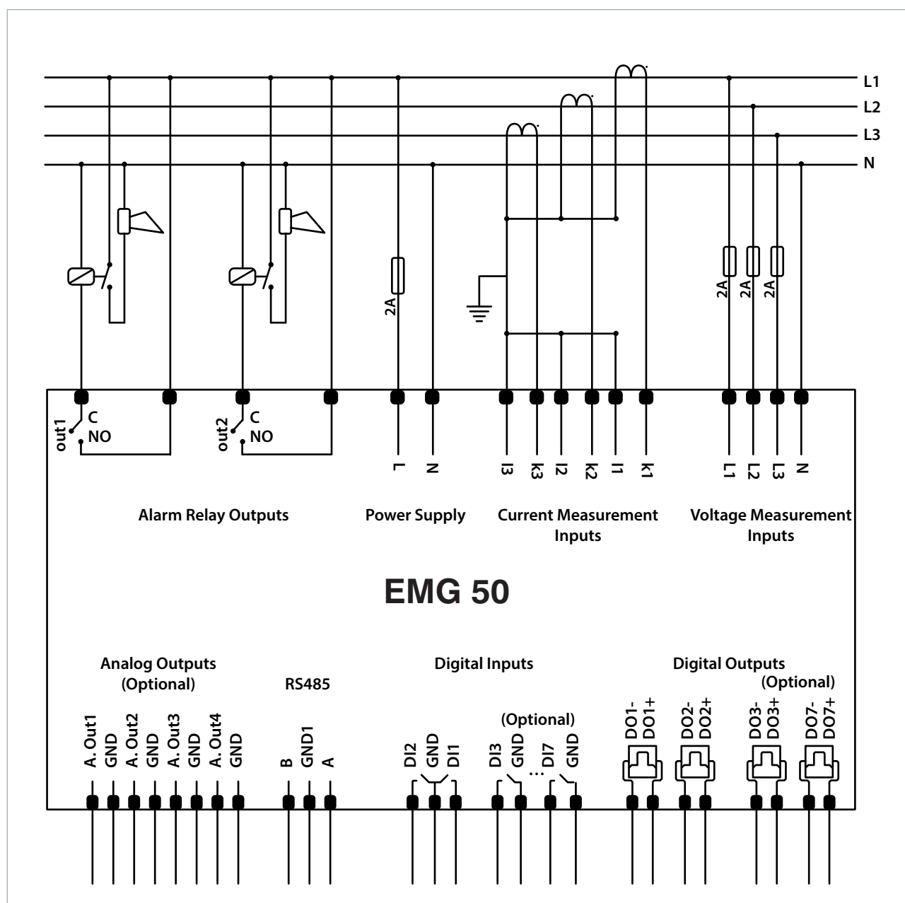
Figure 2-6 EMG 50 Star (WYE) Connection Diagram
