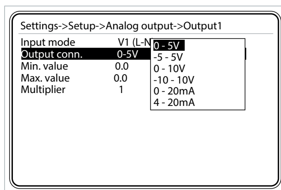
Figure 3-40 Output connection
