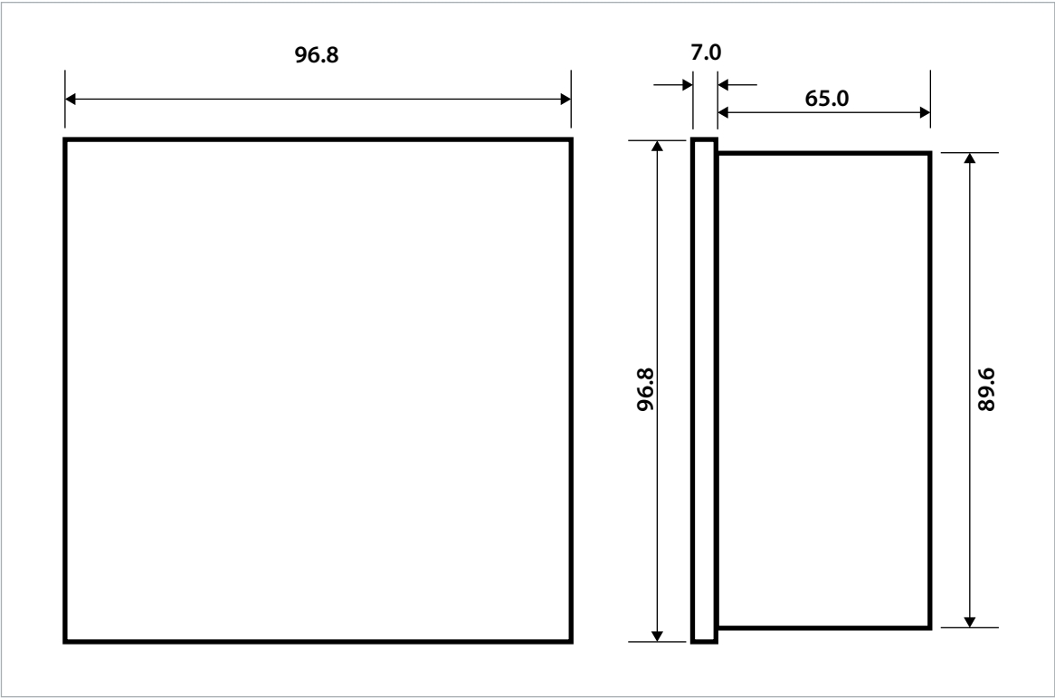
Figure 2-10 Dimensions
