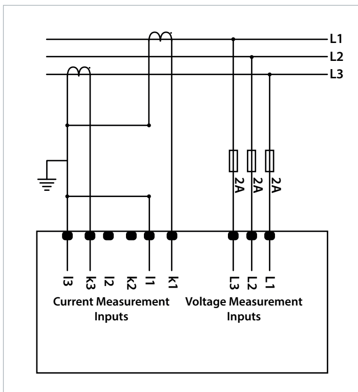
Figure 2-8 EMG 50 Aron Connection Diagram
