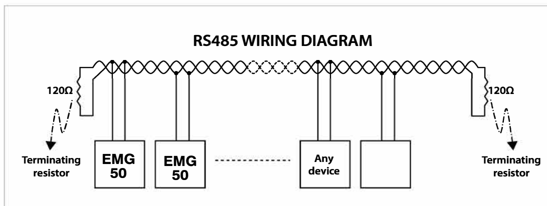
Figure 4-1 RS485 Wiring Diagram
