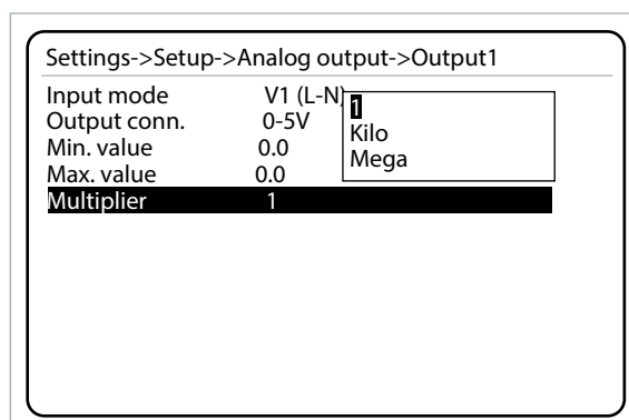
Figure 3-43 Multiplier
