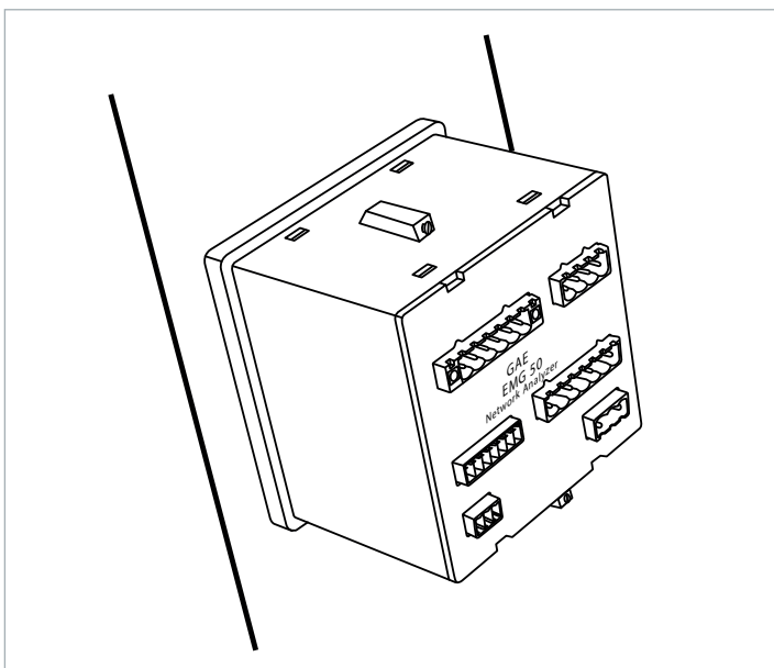
Figure 2-2 Fixing EMG 50 to the panel
