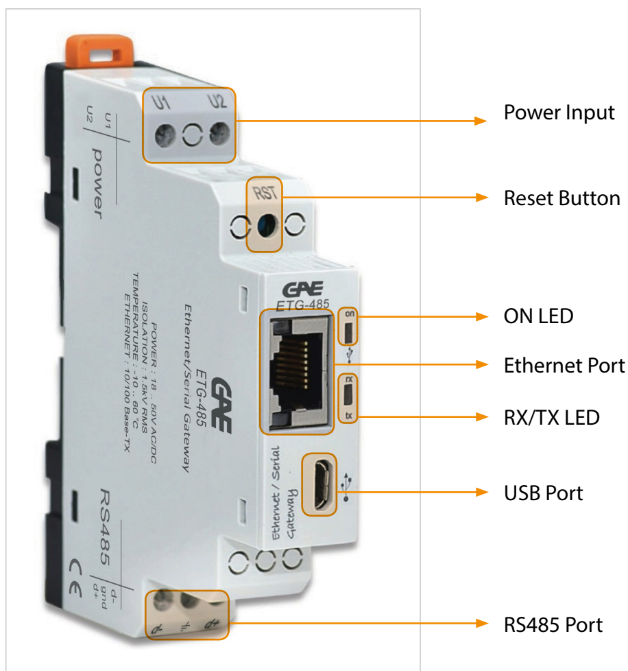
Figure 2-1 Definitions on ETG-485
