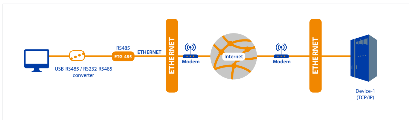
Figure 1-2 General Operating Principle of Client Mode
