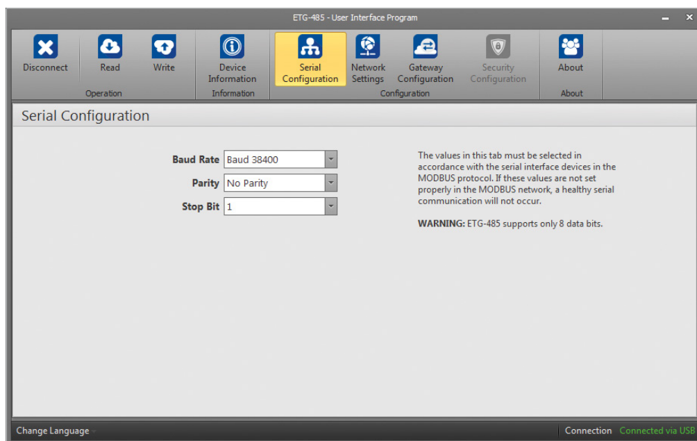
Figure 3-5 Serial Port Settings
