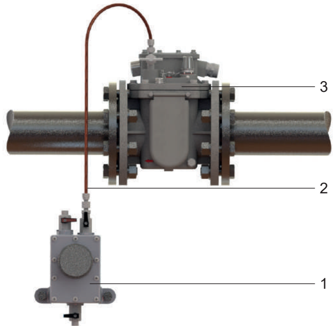
Figure 33 - Mounting of the gas sampling device ZG 1.2.
