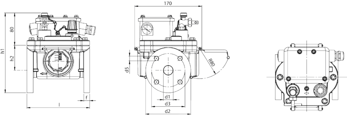
Figure 12 - Dimensional drawing, type 25
