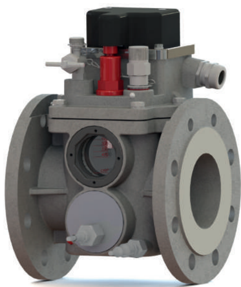
Figure 30 - Buchholz relay type 26 with gas volume sensor – NM series
